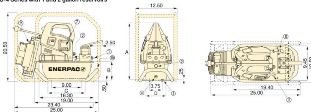
ZU-4 Series with 1 and 2 gallon reservoirs
