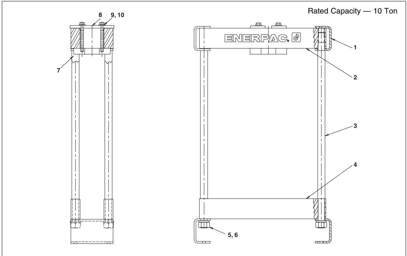
Figure 1, 10 Ton Press Assembly
