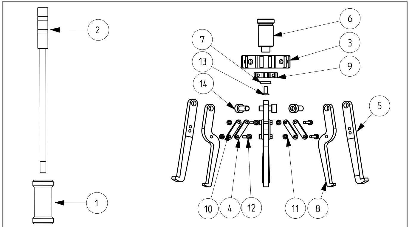
Figure 1, Mechanical Internal Puller Assembly, IPM3
