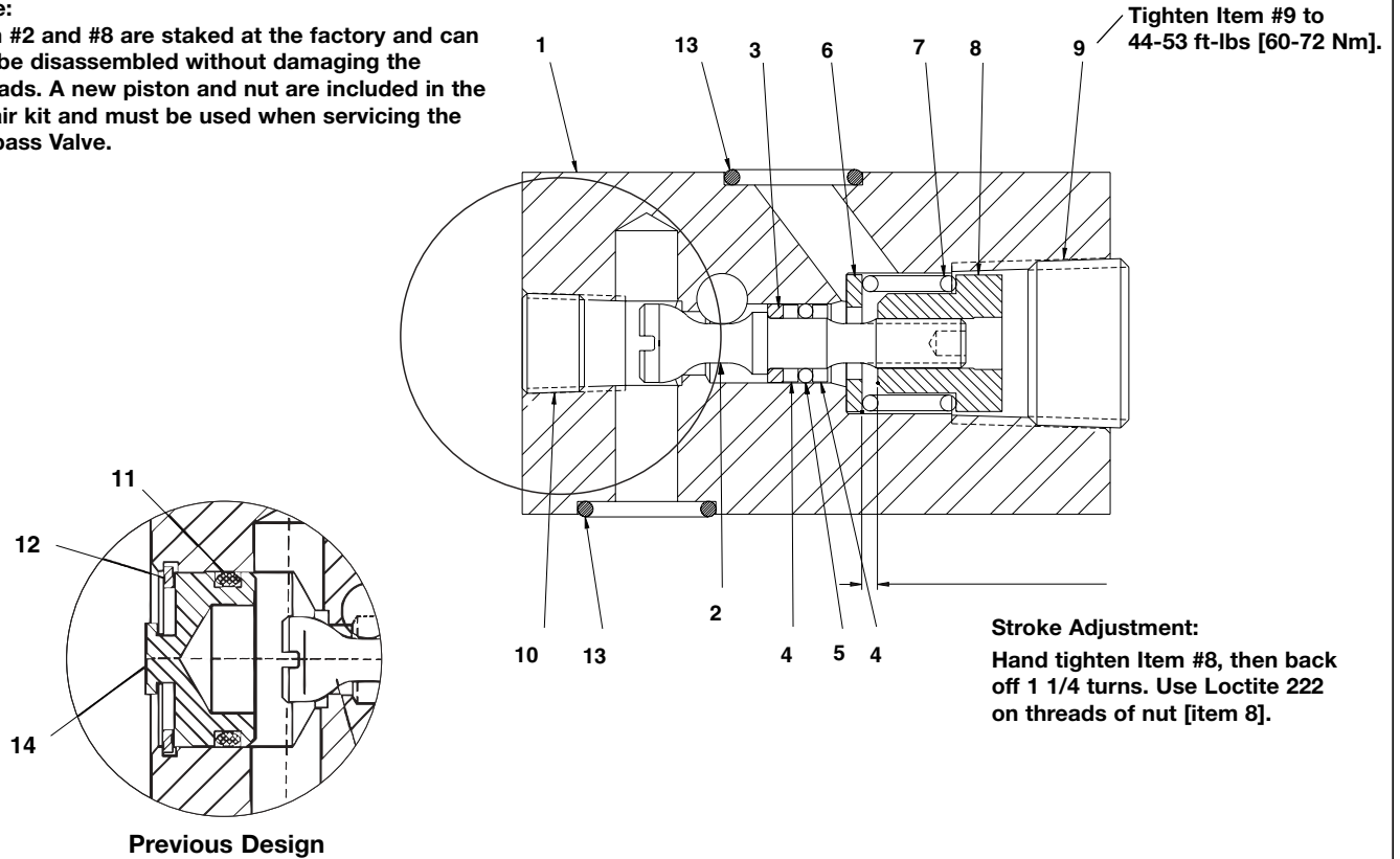
Figure 2B, Bypass Valve Assembly (Early Models, Date Code "A")
