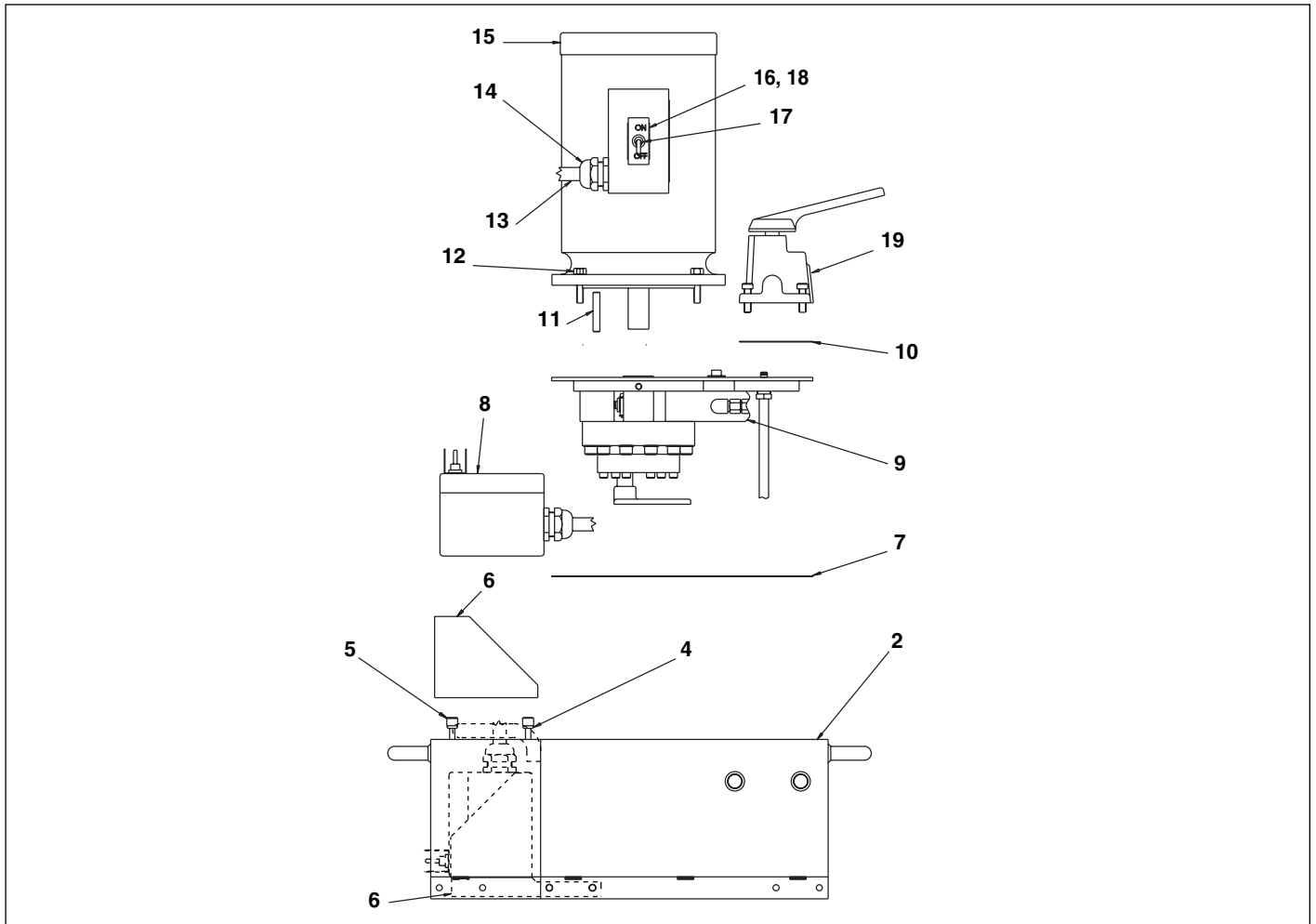
Figure 1, Pump and Reservoir Assembly
