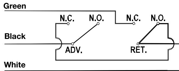
Wiring Diagram
