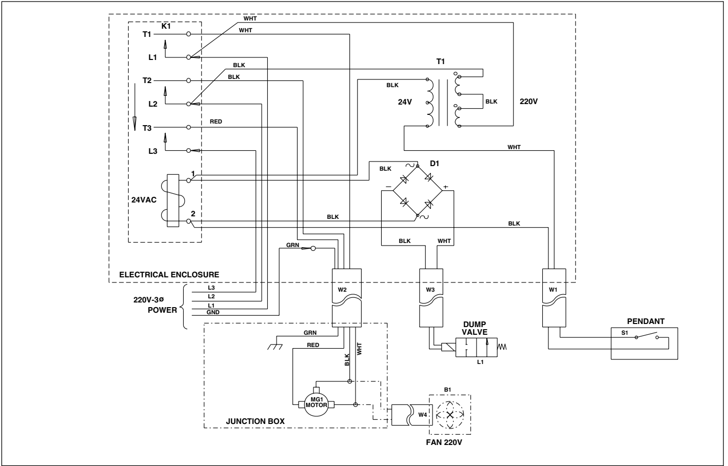
Figure 24, 220-Volt 3-Phase Pump with Dump Valve
