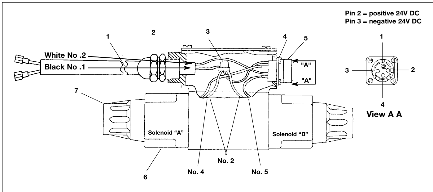
Figure 5C, Solenoid Assembly
