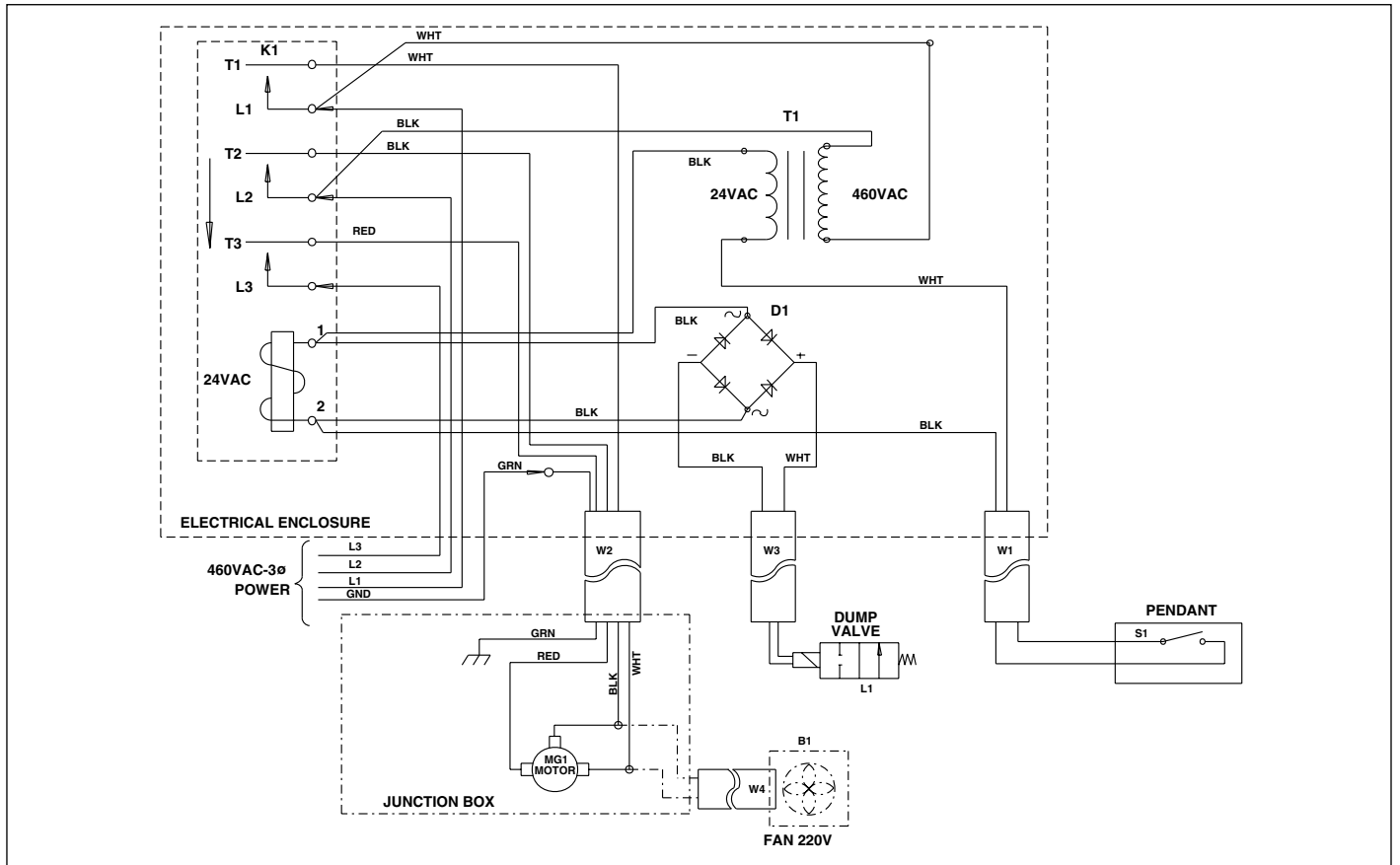
Figure 25, 460-Volt, 3-Phase Pump with Dump Valve
