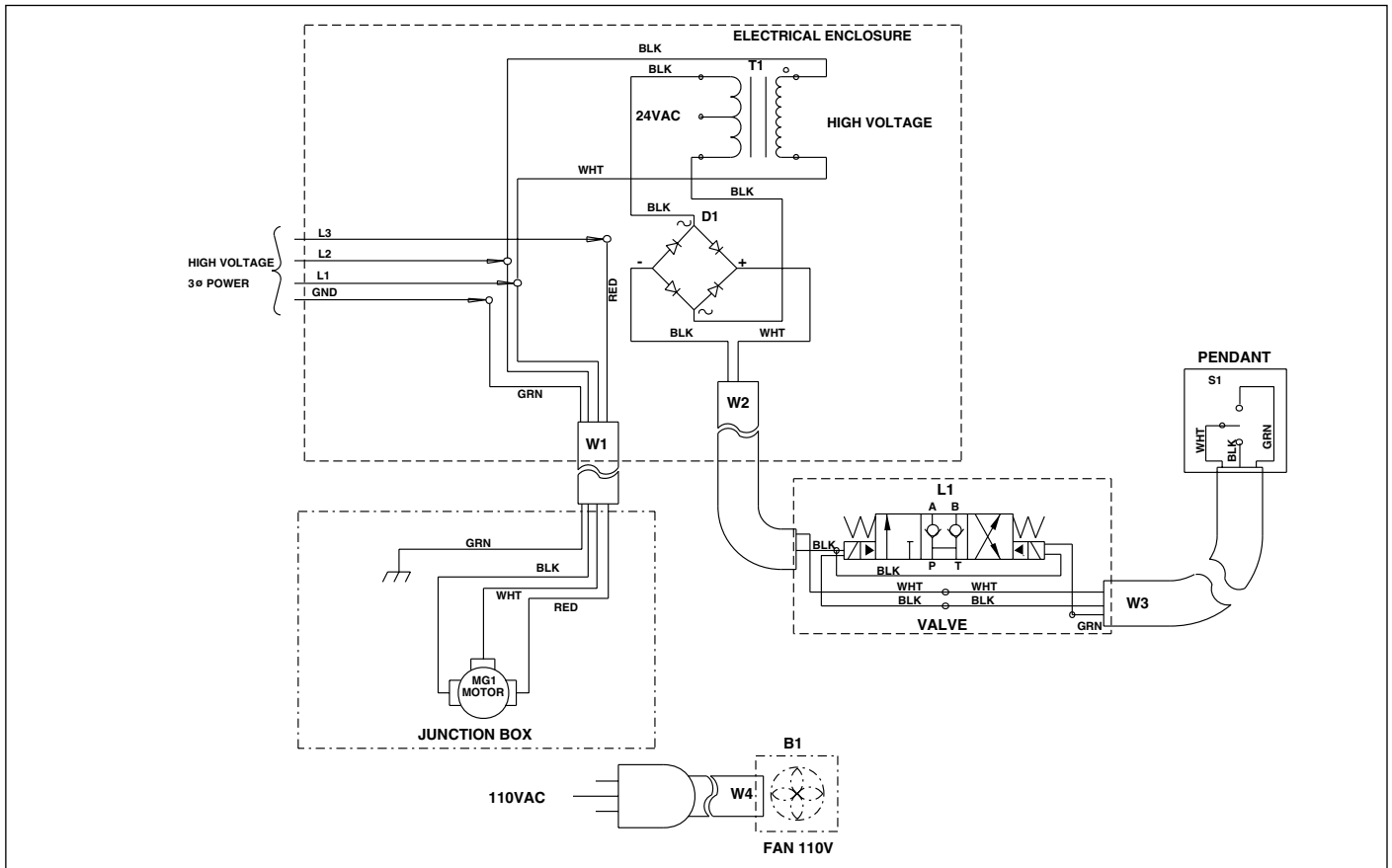
Figure 21, 460/575-Volt, 3-Phase Pump with 4-Way Electric Solenoid Valve
