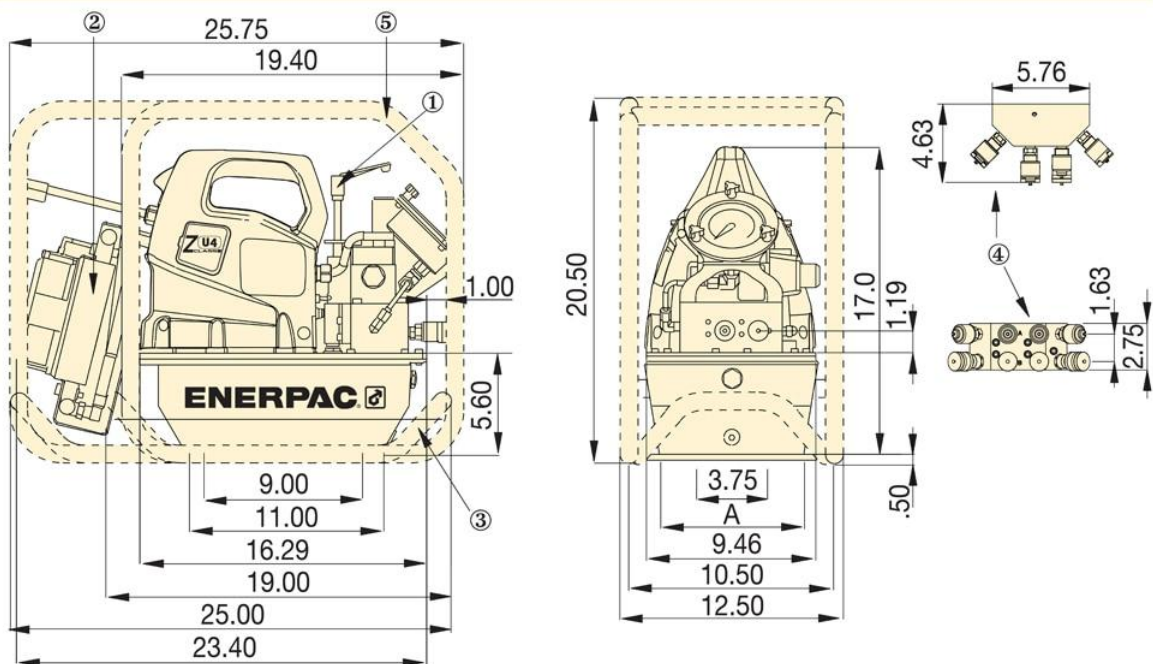
ZU4-Series Torque Wrench Pumps
