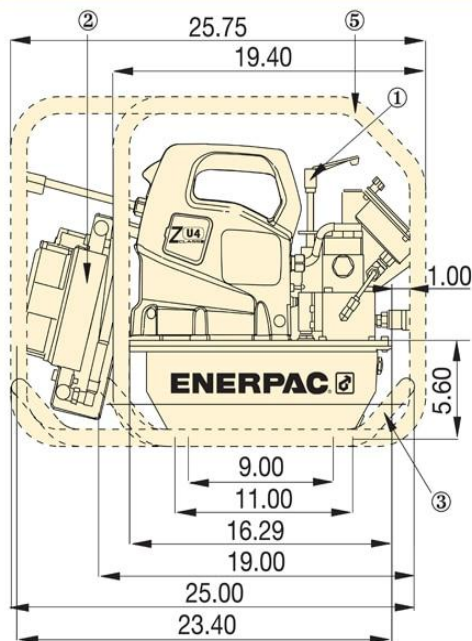
ZU4-Series Torque Wrench Pumps
