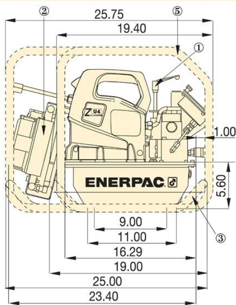
ZU4-Series Torque Wrench Pumps
