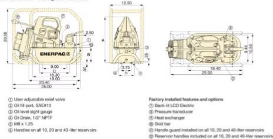
ZU-4 Series with 1 and 2 gallon reservoirs
