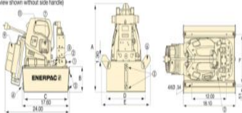
ZU-4 Series with 2.5, 5.0 and 10.0 gallon reservoirs (Left view shown without side handle)
