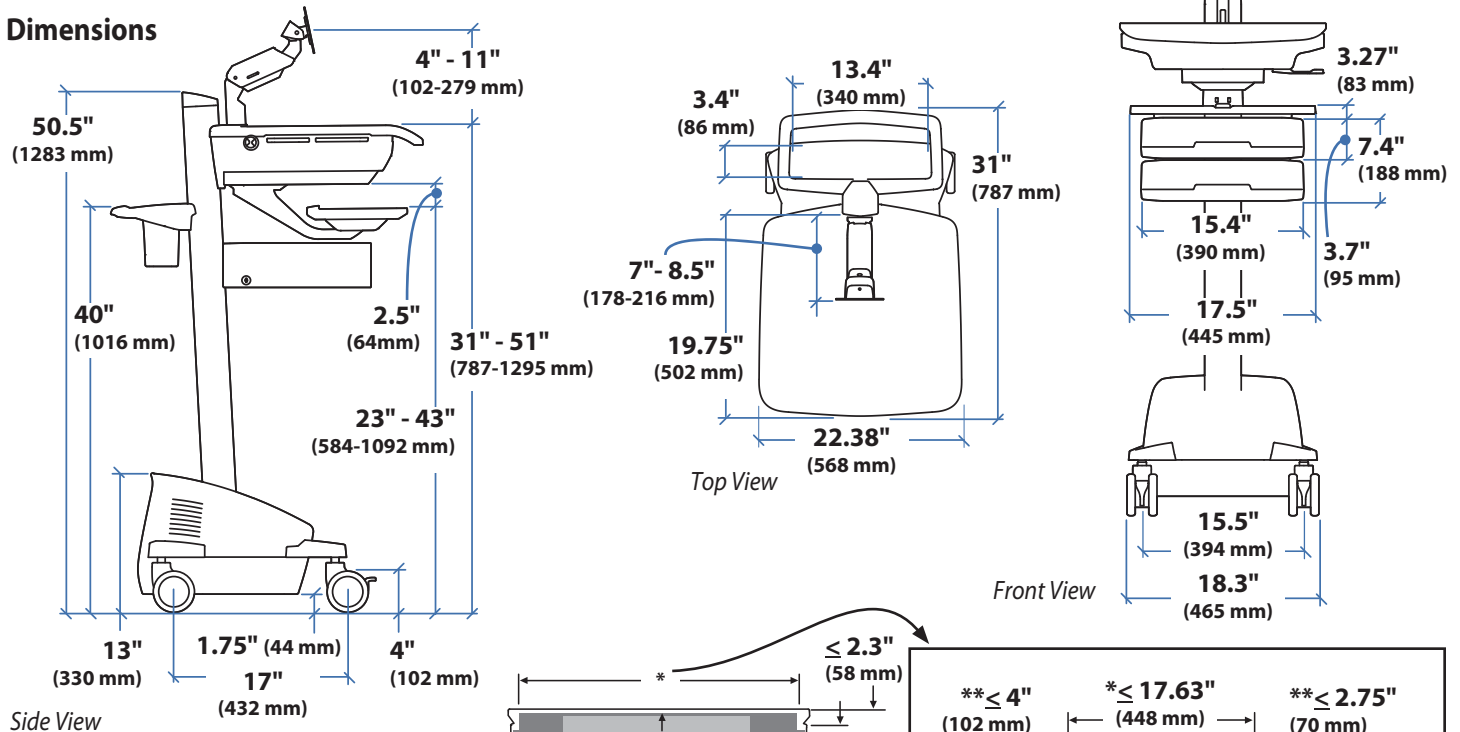
Side View
