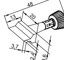
0102WDLF35/SB PowerWell with concave portion, 3.5 mm \emptyset
