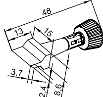
0102WDLF23/SB PowerWell with concave portion, 2.3 mm \emptyset
