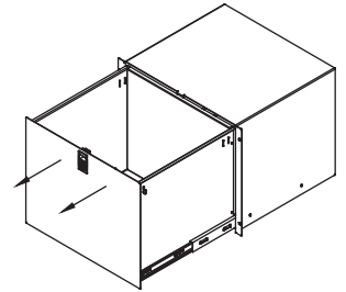
Locking File Drawer (8RU) w/ file holder interior dims: 15 \frac{3}{4} "W x 13 \frac{9}{16} "D x 13 \frac{5}{16} "H (50 lbs max load) 97515
