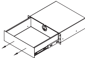
Drawer (3RU) interior dims: 15 \frac{15}{16} "W x 14 \frac{1}{2} "D x 5 \frac{1}{4} "H (50 lbs max load) 97518
