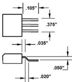
500-13A-US Flat Pack Forming (Gull wing Bend)
