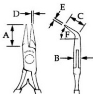
2629 Bent Nose Pliers Smooth Jaw
