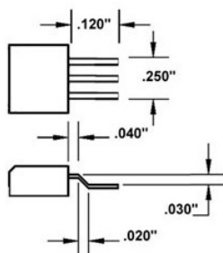
500-13B-US Flat Pack Forming (Gull wing Bend)
