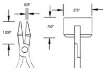
508-US Straightening Pliers with ESD Safe Delrin Jaws
