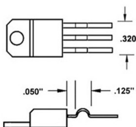
554AJ-US Component Forming "Stress Relief Bender"
