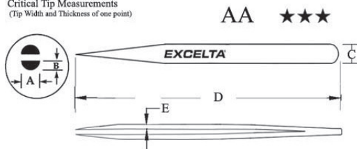
C.T.M. Critical Tip Measurements (Tip Width and Thickness of one point)
