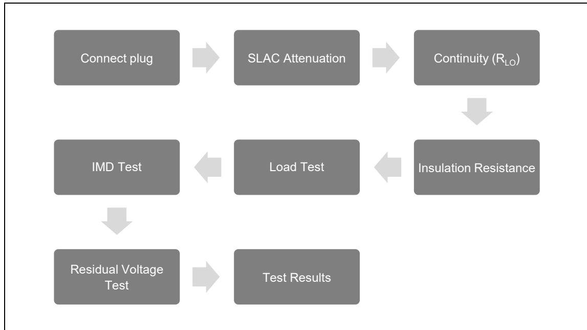
Figure 3. Project Setup
