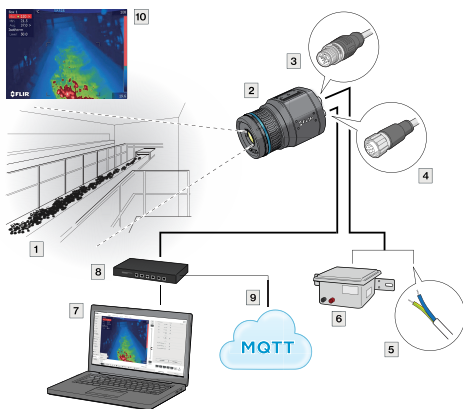
Figure 2.5 Example system overview: early fire detection
