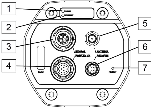
Figure 2.1 View from the rear: FLIR A400/A700
