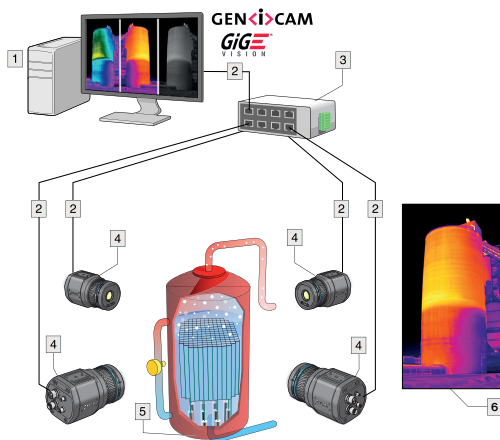
Figure 2.6 Example system overview: condition monitoring
