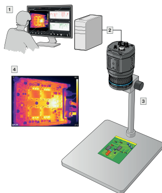
Figure 2.7 Example system overview: research and development
