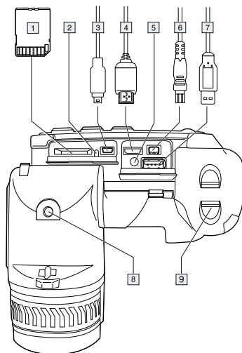
Figure 2.4 View from the bottom
