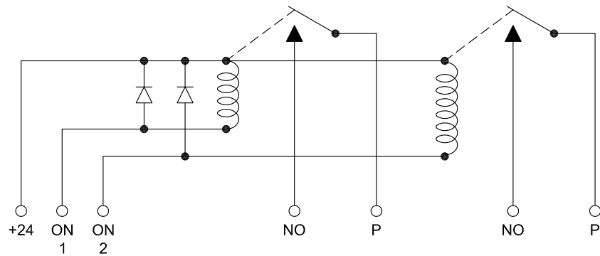
SCHEMATIC DIAGRAM AC-2
