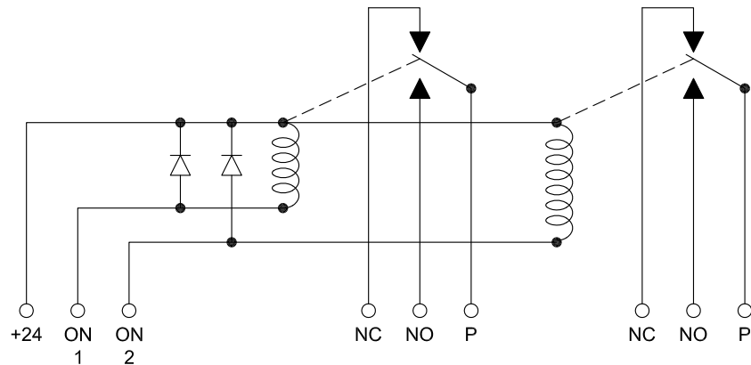
SCHEMATIC DIAGRAM AC-2A
