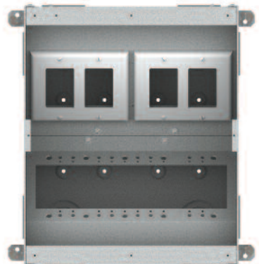
Plate Configuration 2-2
