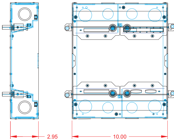
FL-500P-3-B 3" Deep
