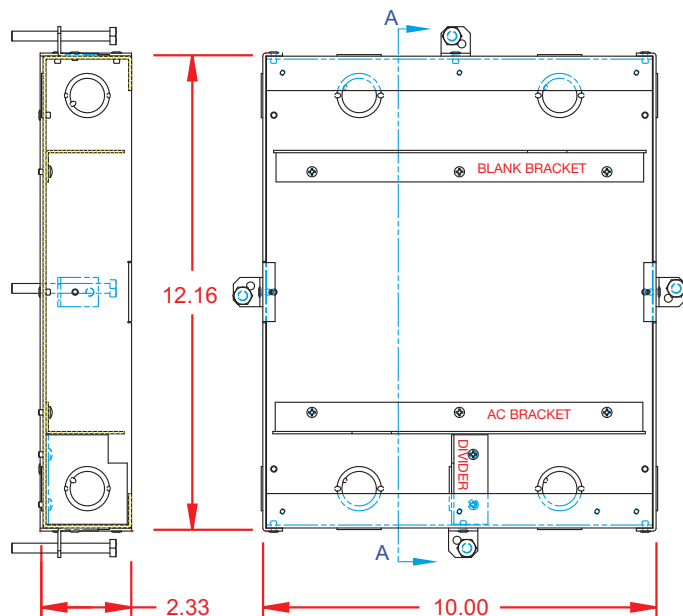
FL-500P-2.25-B 2.25" Deep
