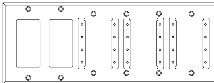
IPS-WP2H 3 IPS & 2 Decora Openings
