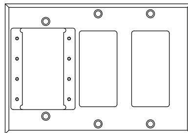
IPS-WP3T 1 IPS & 2 Decora Openings
