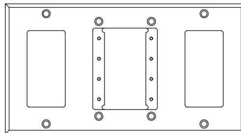
IPS-WP4Q 1 IPS & 2 Decora Openings
