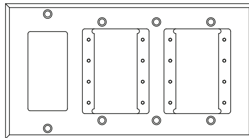
IPS-WP3Q 2 IPS & 1 Decora Opening
