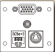
IPS-AVC942T HD15 to 5 BNC's, 3.5mm Stereo to Solder, RJ-45, S-Video
