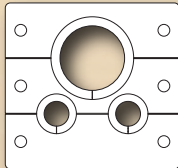
IPS-B030T 2 x .312" and 1 x .812" Split Bushing
