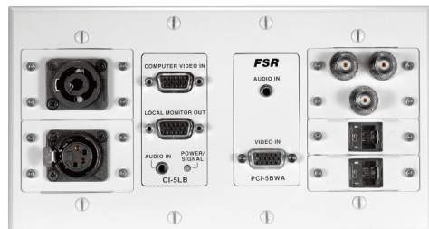
IPS-WP2Q-WHT (populated)
