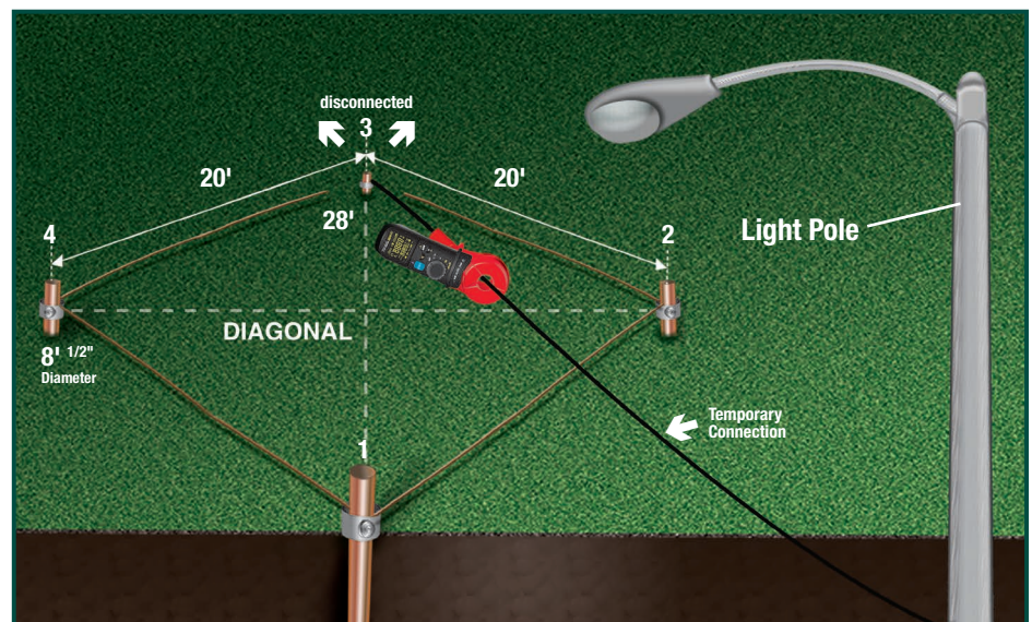
Figure 6 Single rod test using the Model 6417 Clamp-on Ground Resistance Tester
