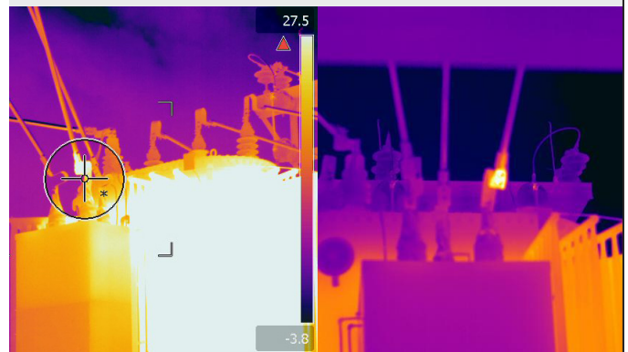
Through regular inspections, maintenance professionals can rapidly detect and locate temperature issues of electrical components and equipment.
