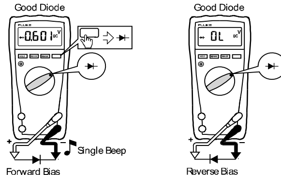
Forward Bias
