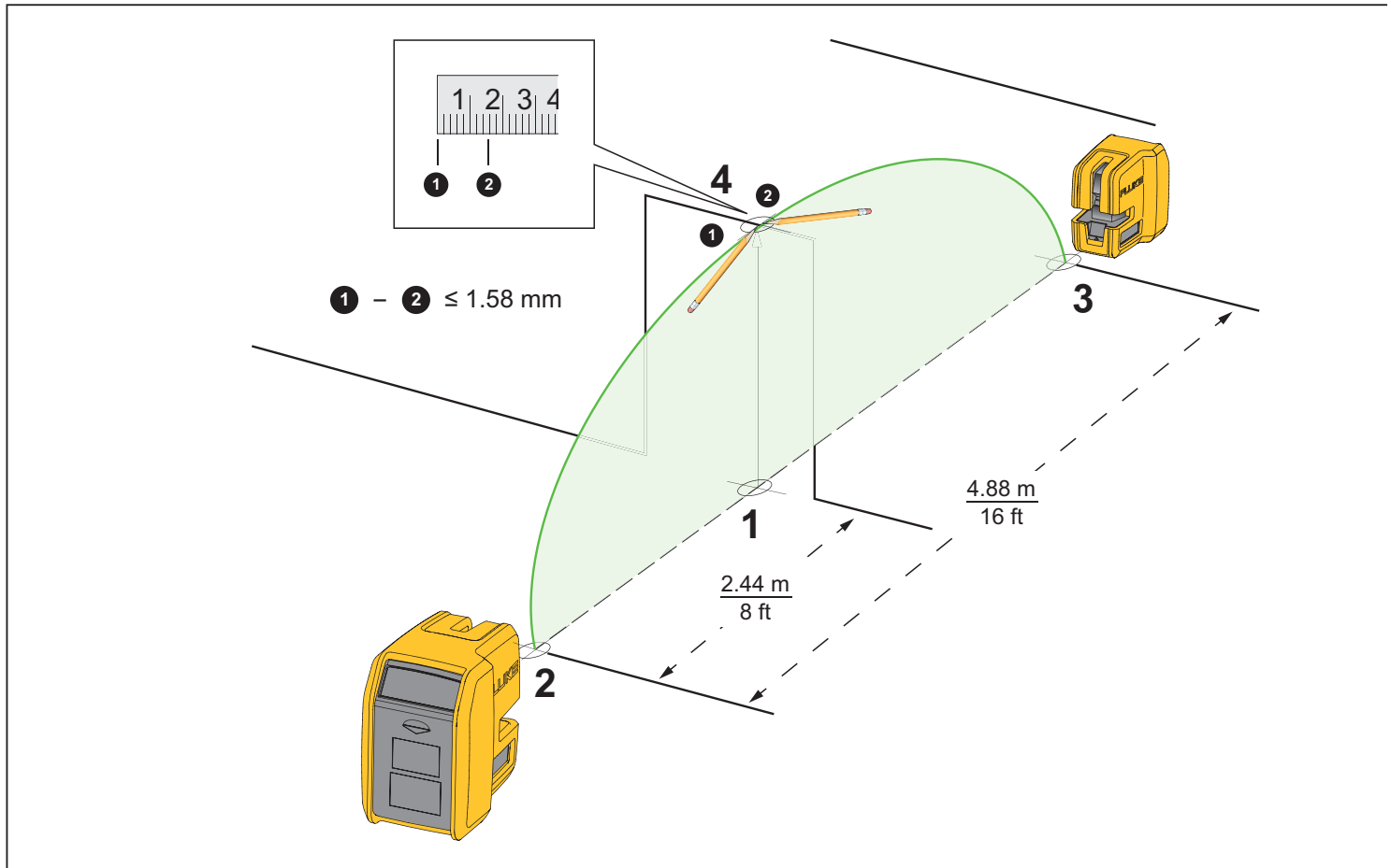
Figure 6. Vertical Laser Accuracy
