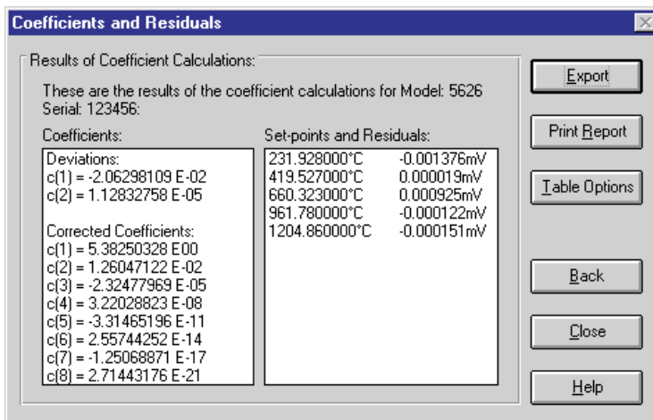
Figure 19 Coefficients and Residuals dialog
