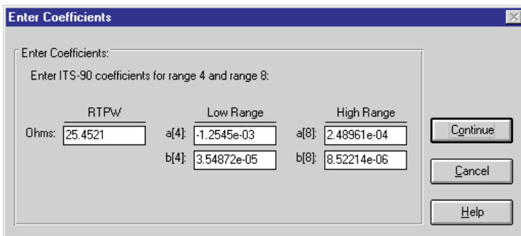
Figure 30 Enter Coefficients dialog for ITS-90 coefficients
