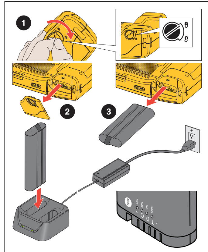
Figure 1. Battery
