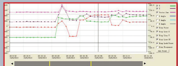
A typical 3-axis vibration data log
