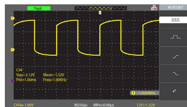
Figure 7. Under Compensated
