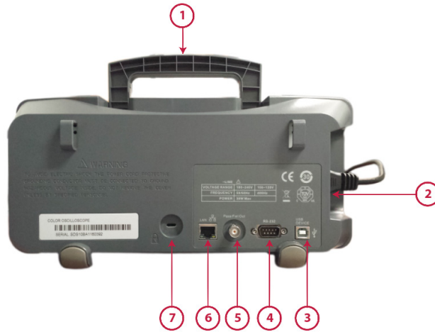
Figure 2. Rear Panel
