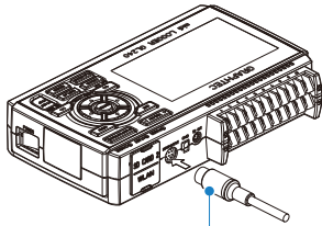
Input/output cable for GL (B-513: Option)
