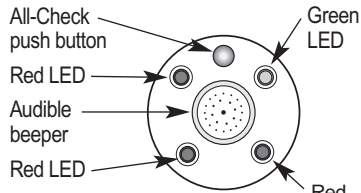
Figure 3 TAG-330 Control Panel
