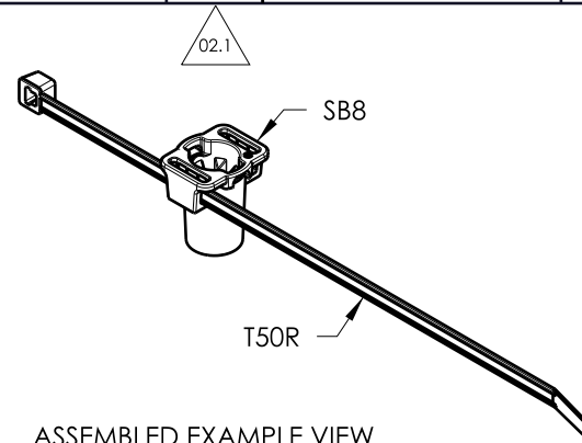
ASSEMBLED EXAMPLE VIEW OPTION 2 SCALE 1:2
