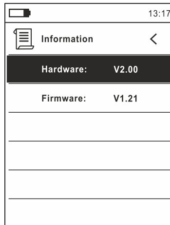
Fig. 12: Menu Information
