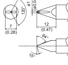
TX1-XRK Shape-XRK
