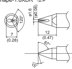
TX1-XDR16 Shape-1.6XDR
