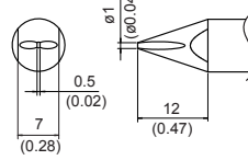
TX1-XD3 Shape-3XD
