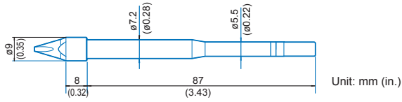
TX1-XD16 Shape-1.6XD
