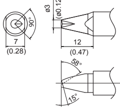
TX1-XDR24 Shape-2.4XDR
