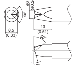
TX2-XRK Shape-XRK
