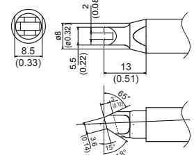
TX2-XRK Shape-XRK
