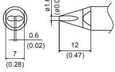
TX1-XBCR3 Shape-3XBCR
