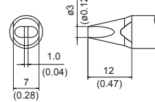
TX1-XDR Shape-XDR
