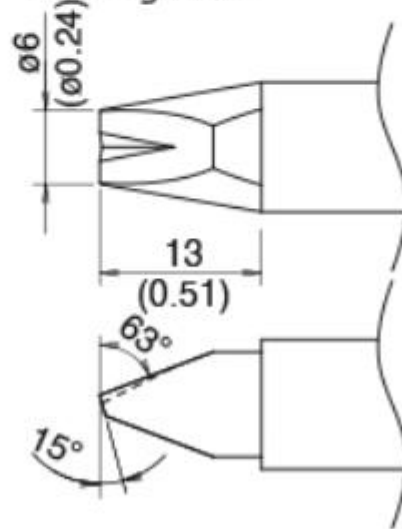
Shape-6XD with V-groove
