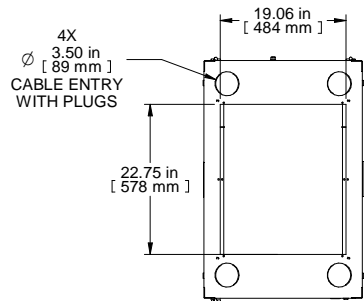
TOP OPENING PLATE REMOVED
