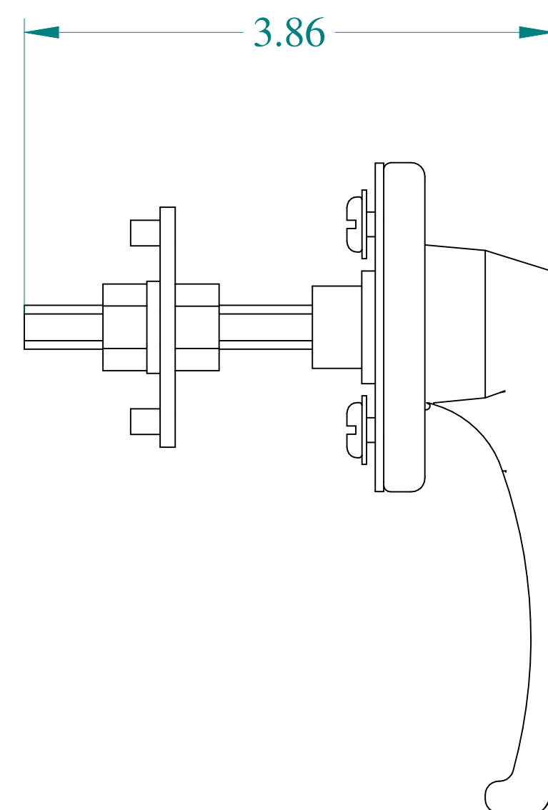
SIDE VIEW
