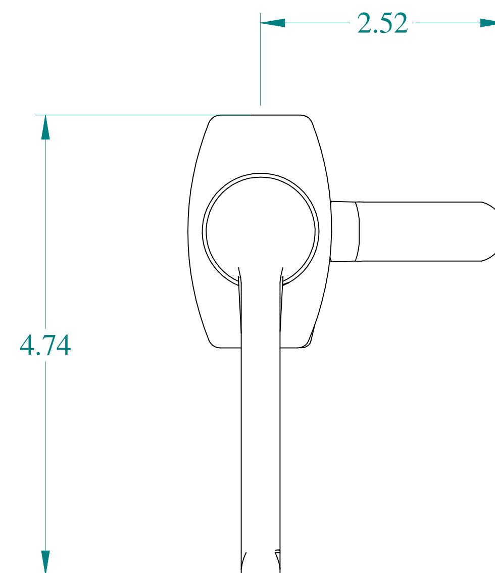
FRONT VIEW
