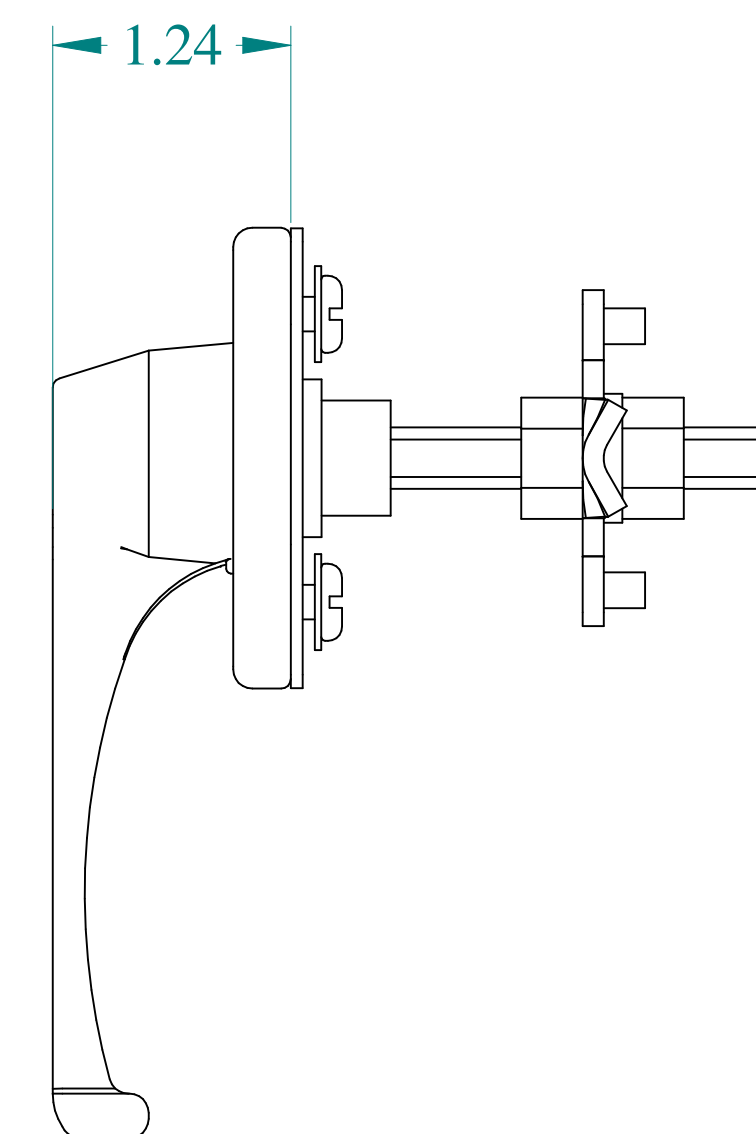
SIDE VIEW
