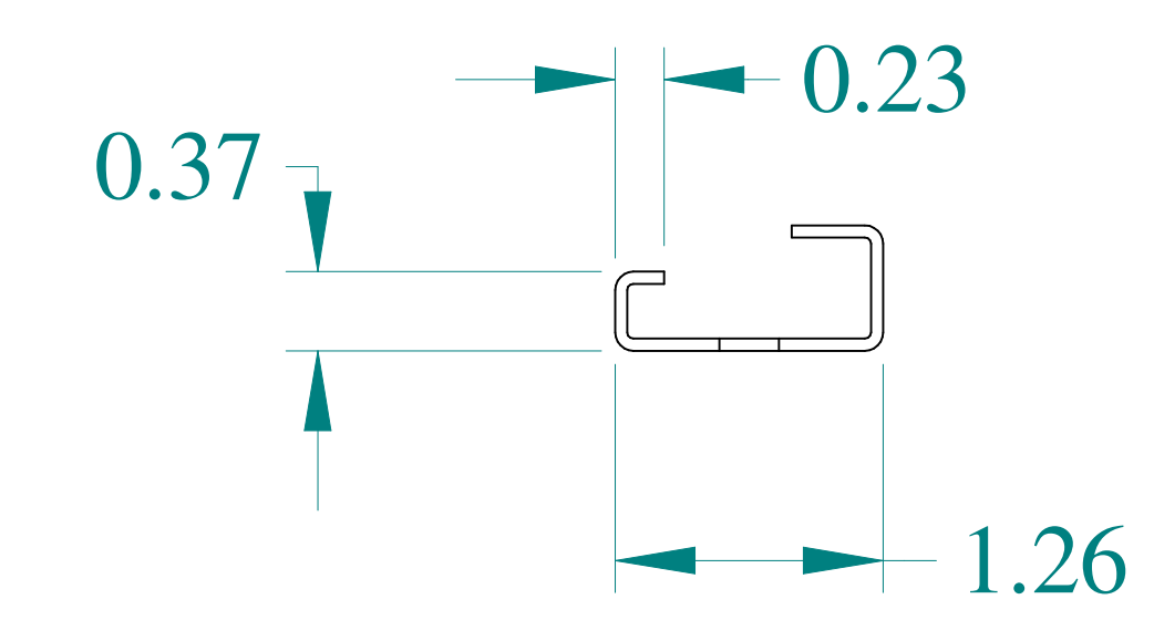
SIDE VIEW
