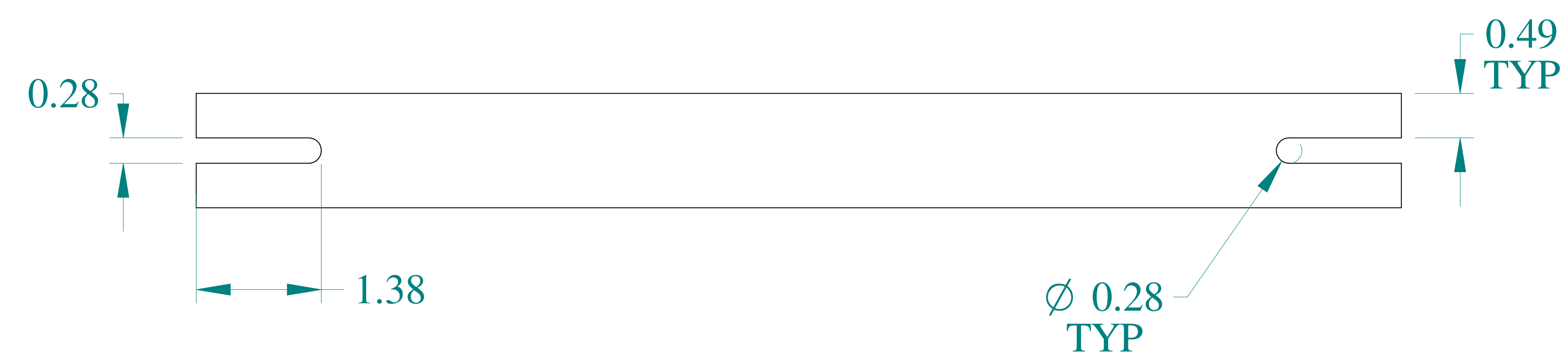
BOTTOM VIEW
