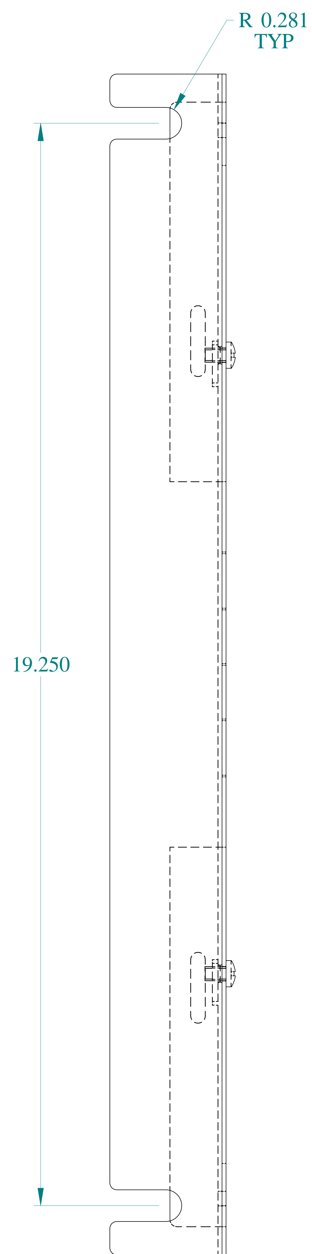
SIDE VIEW
