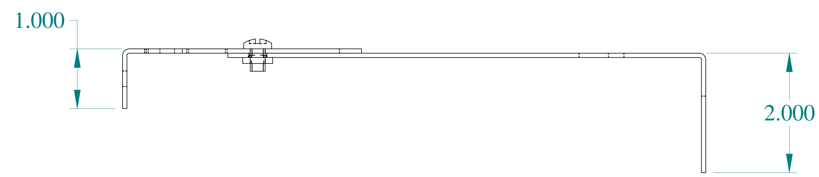
TOP VIEW
