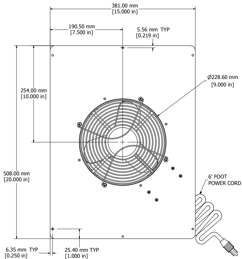
ASSEMBLY - VIEW FROM TOP
