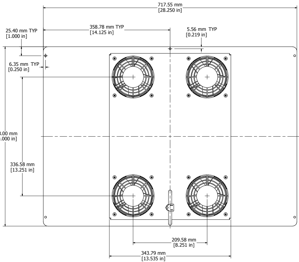
ASSEMBLY - VIEW FROM BOTTOM
