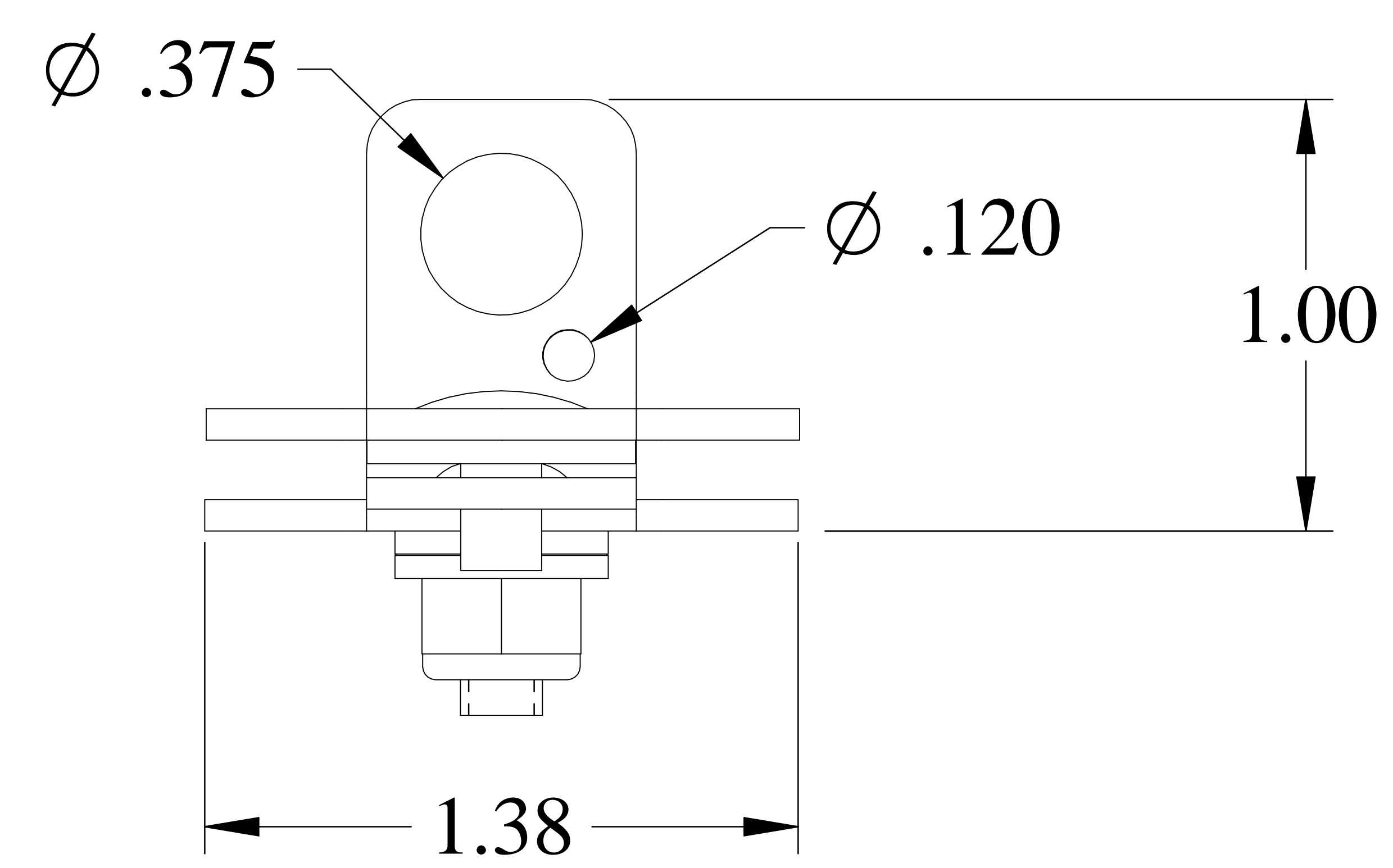
FRONT VIEW
