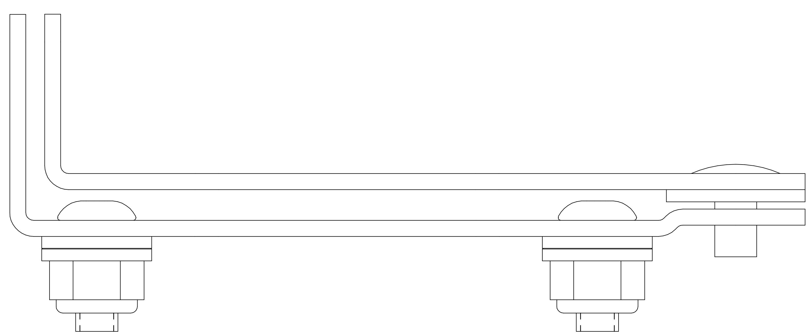
SIDE VIEW
