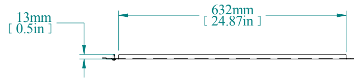
TOP VIEW
