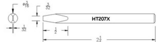
Conical Chisel (Standard)
